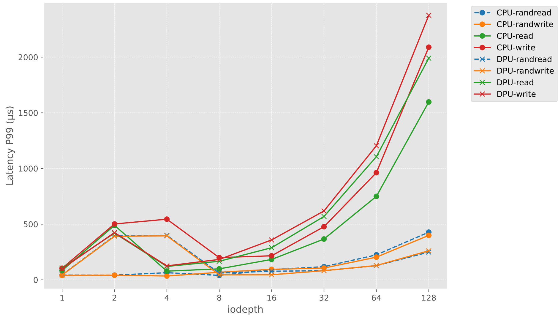
Latency P99 vs iodepth
